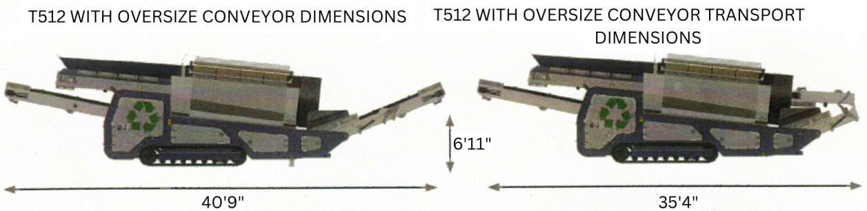
T512W WITH OVERSIZE CONVEYOR DIMENSIONS T512 WITH OVERSIZE CONVEYOR DIMENSIONS
